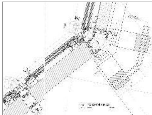
Unitized curtain wall - horizontal section
